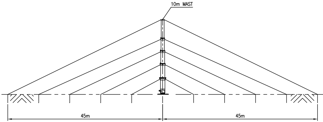
ERECTED POSITION
